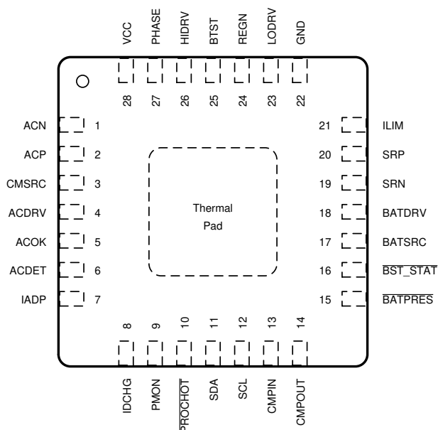
Figure 4-1. RUY Package 28-Pin WQFN Top View
