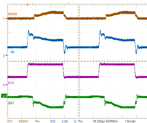
Figure 7-13. Converter in Discontinuous Conduction Mode During Hybrid Power Boost Mode
