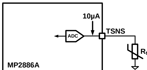
Figure 10: Temperature Sense for MP2886A with Thermistor
