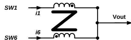
Figure 17: Couple Inductor Connection
