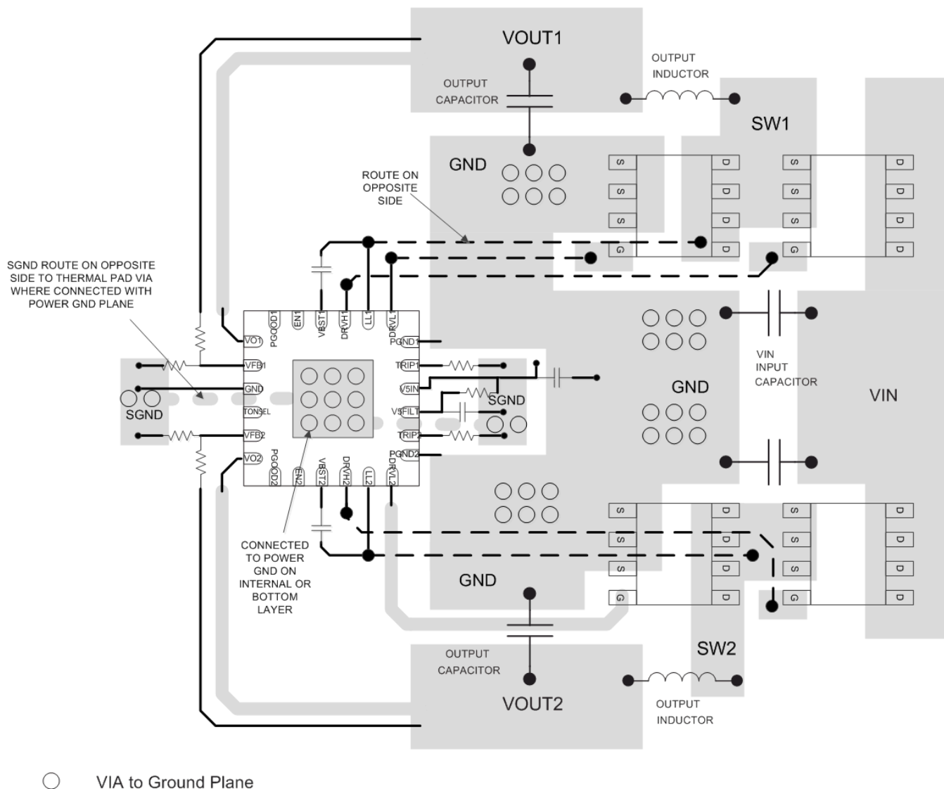
Figure 26. Layout Example
