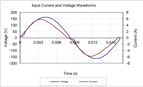
Input AC Current Waveform (ITHD = 12.61%, 50% Load)
